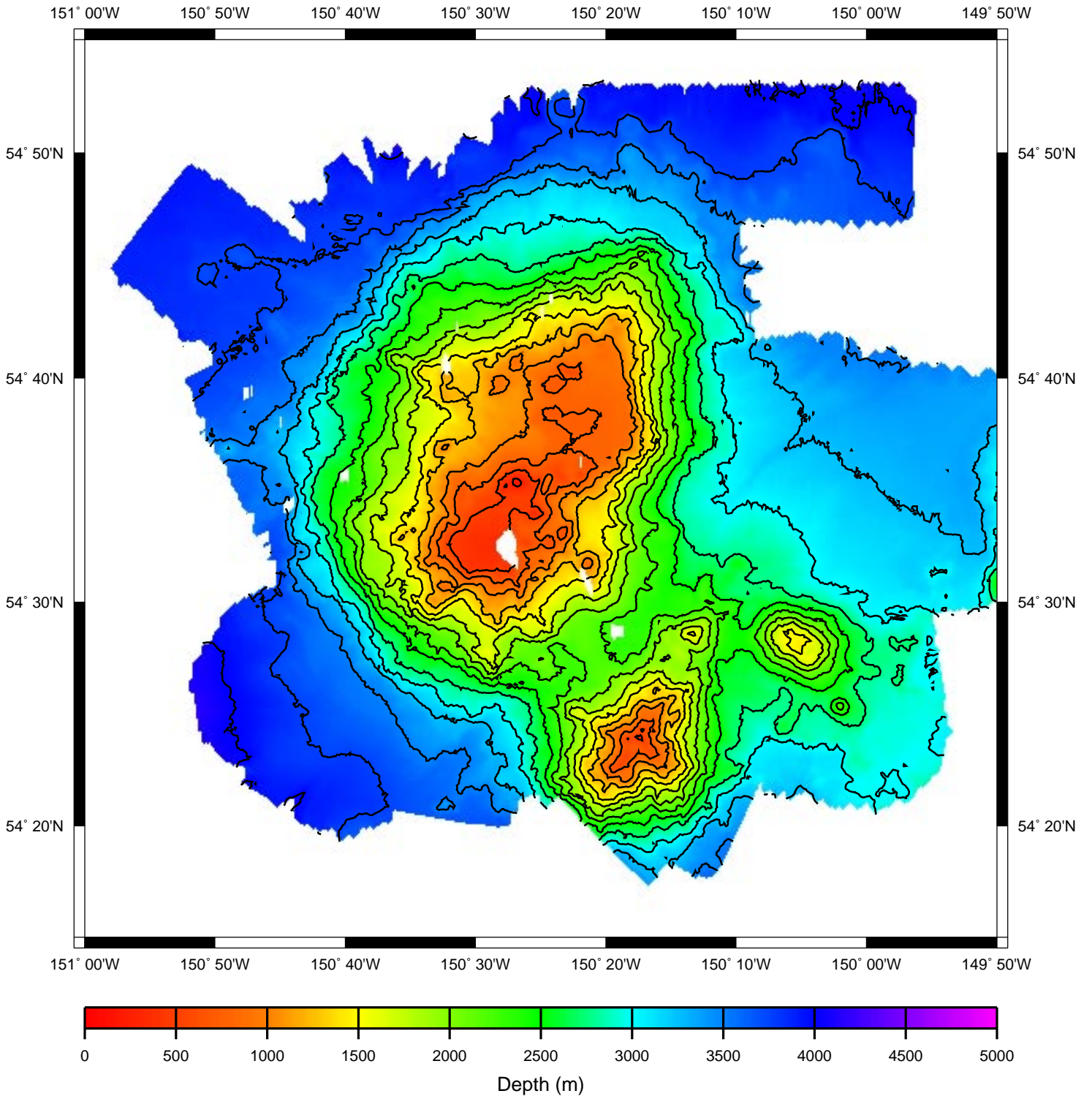
File Patton150.grd - Bathymetry Grid
